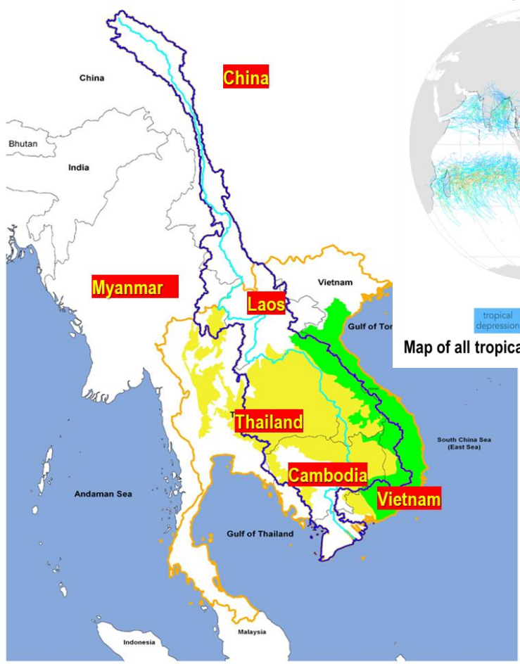
Mekong River watershed
