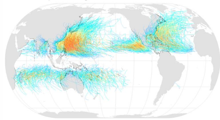
Saffir-Simpson Hurricane Scale:
